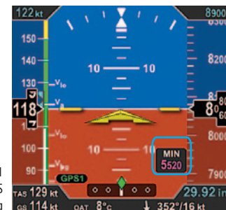
Figure 4-31 New Selected MINIMUMS Annunciation Setting
